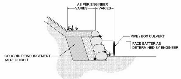
Figure 10.3. Engineering Design Drawing for Filtrexx MSE GreenLoxx™ Headwall Application
