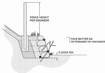
Figure 10.2. Engineering Design Drawing for Filtrexx MSE GreenLoxx™ Fence Detail
